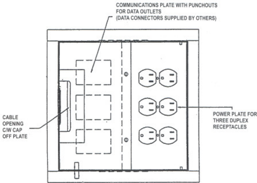
PLAN VIEW
