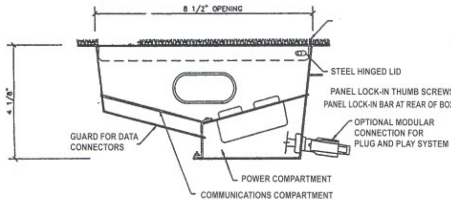
END VIEW
